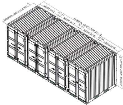
(4) Quadcon Containers coupled together to form one 20' ISO Module
