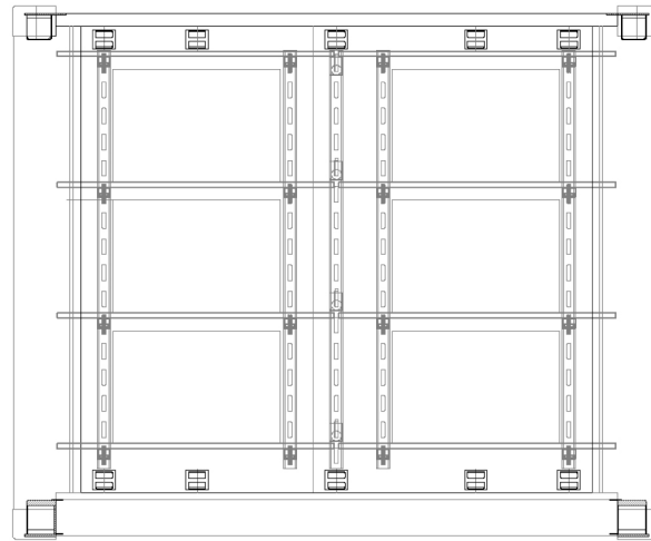
INTERIOR CURB SIDE ELEVATION
