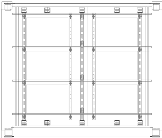
INTERIOR ROAD SIDE ELEVATION
